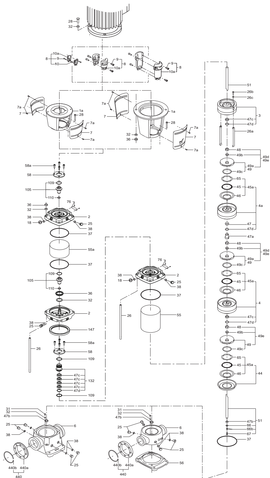
Exploded view for CR, CRI, CRN 32, 45, 64, 90, model A, back to back
