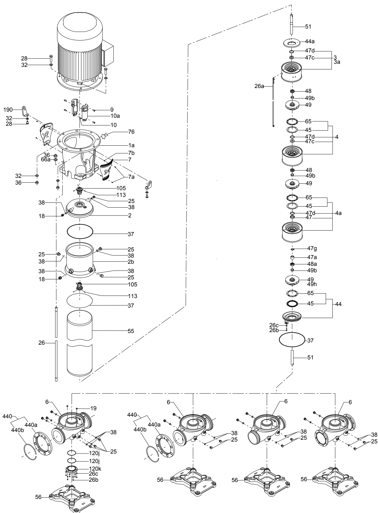
Exploded view for CR, CRN 95 - 255, ø28 or ø36 back-to-back shaft seal
