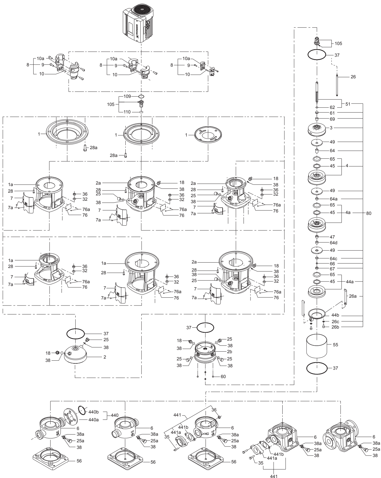
Exploded view for CR, CRI, CRN 10, back to back
